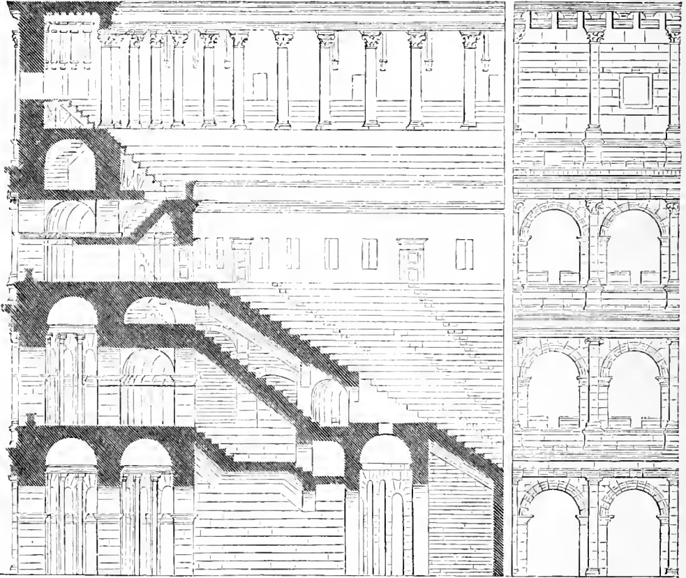
FIG. 132.—THE COLOSSEUM. SECTION AND ELEVATION.
